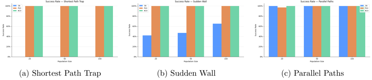
Figure 2: Success rate by population size and maze. GA (blue) solves Parallel Paths, fails the deceptive trap entirely, and partially solves the Sudden Wall with success rising as population grows; the coupled architectures (PSO orange, ACO green) solve all three mazes.
