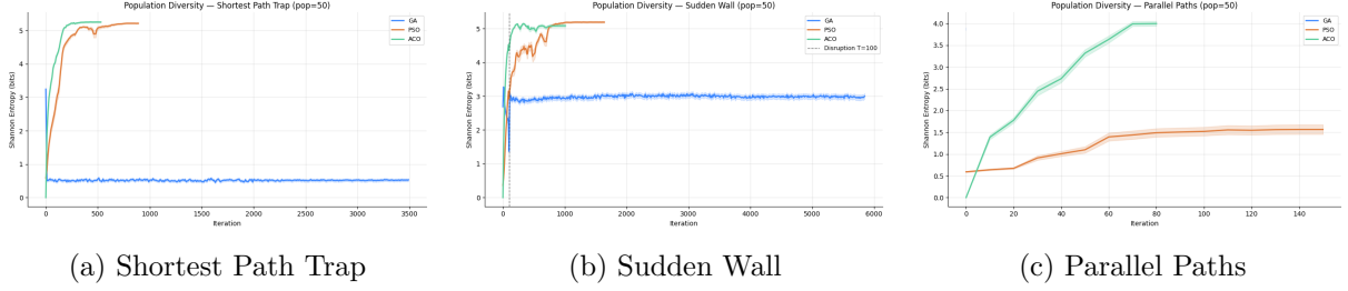
Figure 1: Population diversity (Shannon entropy, bits) over iterations at population 50, with 95% bands across 100 runs. On the deceptive trap (a) and the Sudden Wall (b), ACO (green) and PSO (orange) both climb to a high plateau near 5 bits (ACO faster); GA (blue) collapses to about 0.5 bits on the trap but holds a moderate \sim 3 bits on the wall. The dashed line in (b) marks the disruption at T = 100 . On Parallel Paths (c), PSO sits lowest having collapsed onto a single route, while ACO rises highest; GA is not visible because it solves the maze in its first generation, leaving a single high-entropy point at the left edge rather than a curve.
